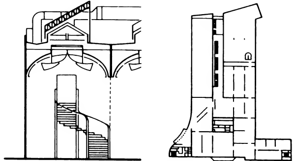
2 Lighting detail
